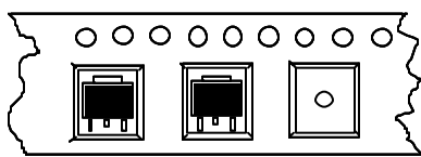
TO252; 263 Package Orientation
