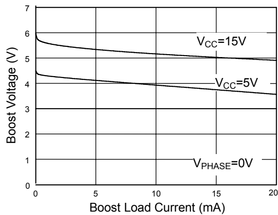
Fig. 6 Boost Load Regulation
